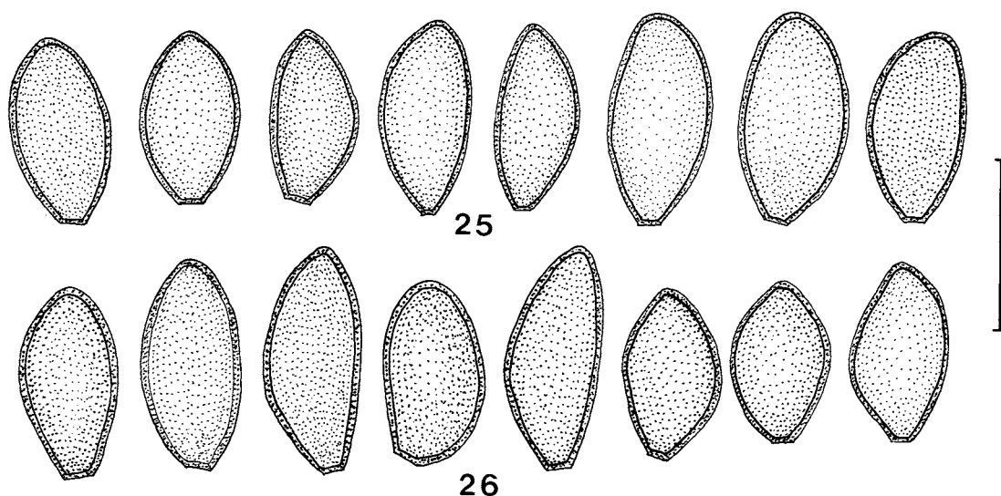
Figs 25–26. Conidia of Pilidiella diplodiopsis . Fig. 25. STE-U 3940 (ex-type). Fig. 26. STE-U 3938. Bar = 10 \mu\text{m} .
